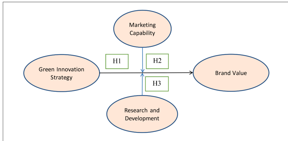
Fig. 1. Theoretical Framework.
